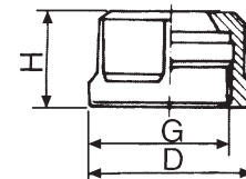
FIG.3 ER11,16,20UM
