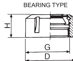
FIG.5 ER40,50KM
