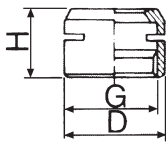
FIG.1 ER11MS
